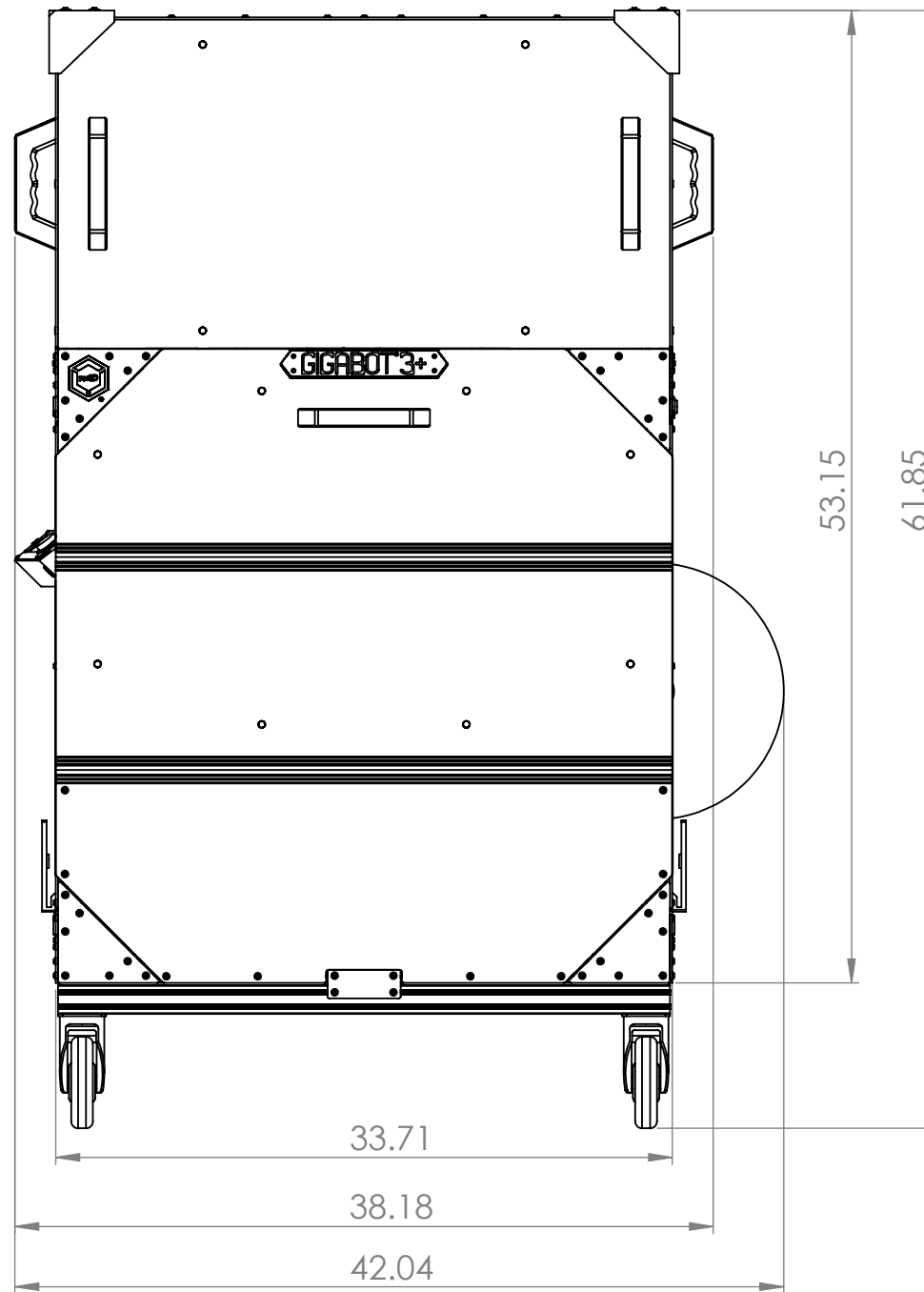
FRONT VIEW
